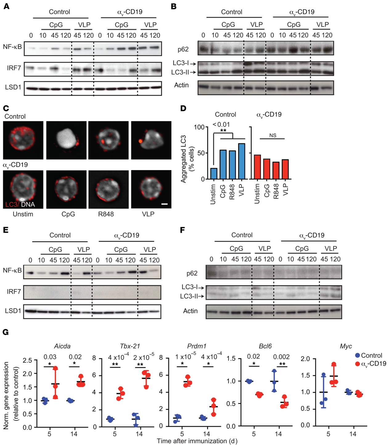
Figure 4. α v Regulates TLR signaling in GC B cells through autophagy proteins. (A and B) GC B cells were sorted from spleens of α v -CD19 and control mice 14 days after immunization with VLP and restimulated in vitro with CpG DNA or VLP for the indicated times (minutes). Western blots show NF-κB p65 and IRF7 in nuclear fractions (A) or p62 and LC3b in whole-cell lysates (B). Also shown is staining of LSD1 or actin to confirm equivalent protein loading in nuclear fraction and whole-cell lysates, respectively. These were performed on the same blot, except in the case of LC3-II, for which actin staining was from aliquots of the same samples run on parallel gels contemporaneously. (C) Confocal images of sorted primary GC B cells (as in A and B) treated with CpG DNA, R848, or VLP for 2 hours and stained for LC3 and Hoescht. Scale bar: 2.9 μm. (D) Quantification of LC3 reorganization after stimulation with indicated TLR ligands. Data are based on analysis of at least 30 cells/condition. P values of less than 0.01 are shown (Pearson's \chi^2 test). *P < 0.05. (E and F) FACS-sorted non-GC follicular B cells from spleens of VLP-immunized α v -CD19 and control mice analyzed as in A and B. (G) Expression of indicated genes measured by quantitative reverse-transcriptase PCR (QRT-PCR) in RNA from FACS-sorted VLP-specific GC cells, isolated 5 or 14 days after immunization with 2 μg VLPs. Data from individual mice are shown, with mean ± SD. P values of less than 0.05 are shown (2-tailed Student's t test). *P < 0.05; **P < 0.005. Data are all from 1 representative experiment of at least 3 independent experiments (2 experiments for p62 blots) in which similar results were seen.
